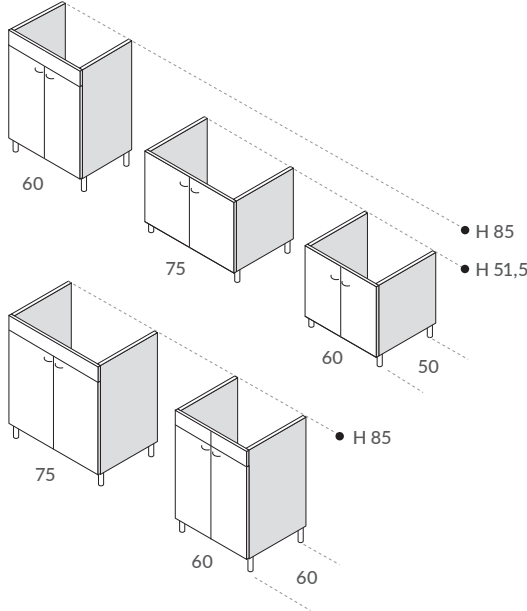
Mobile per lavatoio in ceramica Cabinet for ceramic sink
