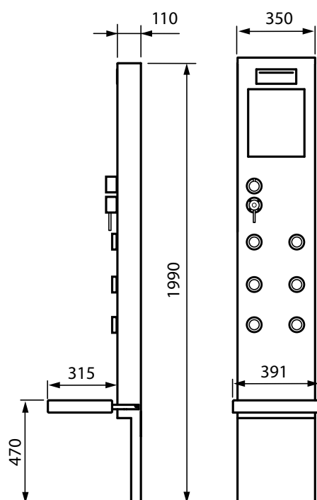
Rigenera 200 (without shower head)
