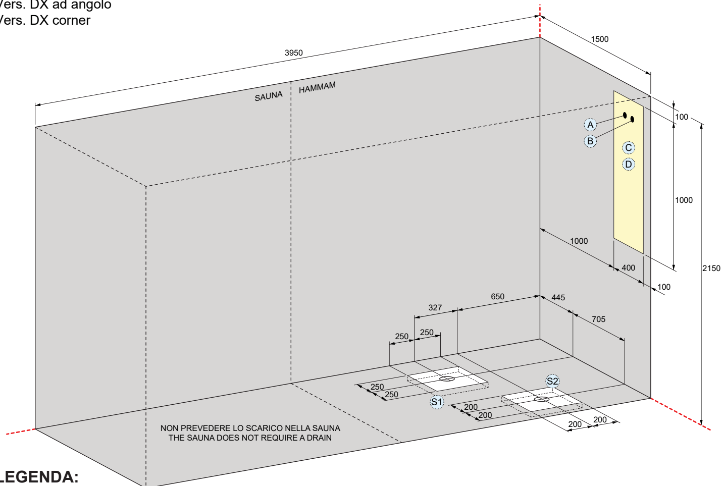
S1: SCARICO VASCA / TAB DRAIN
