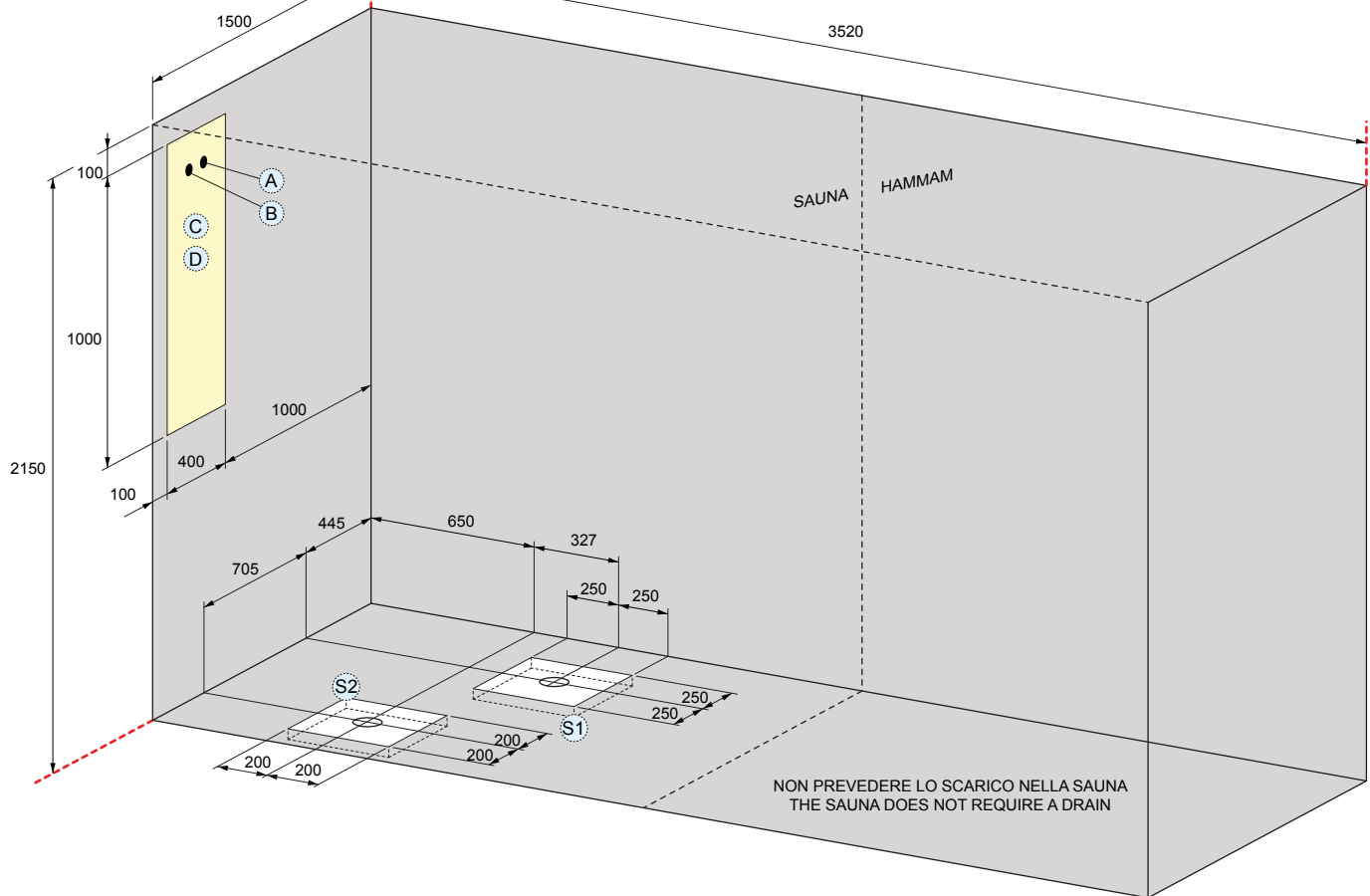
S1: SCARICO VASCA / TAB DRAIN
