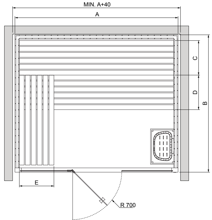
Vers. SX (vista superiore / top view)
