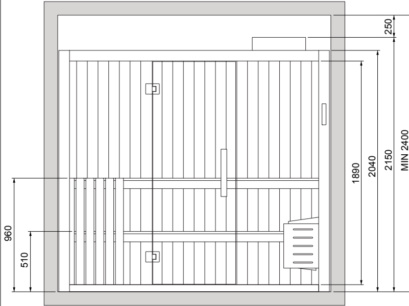
Vers. SX (vista frontale / front view)
